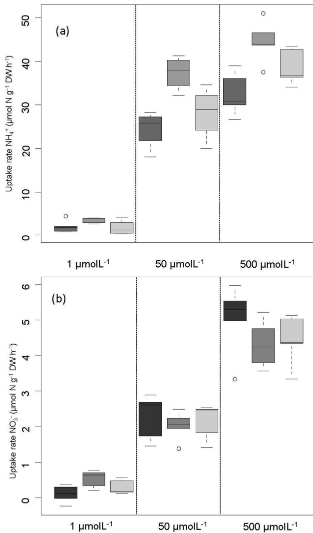
Figure 5. Differences between average uptake rates ( \mu\text{mol N g}^{-1} \text{DW h}^{-1} ) after 0.5 hours in different fractions of Sphagnum magellanicum from the pristine site. We analysed capitula and stems separately, while whole plant values represent the DW weighted mean of both fractions.
